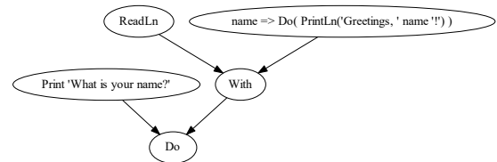
Figure 1. Abstract Syntax Tree of an Imperative Kronos Program
